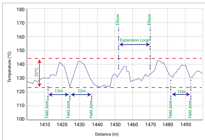
Temperature Profile
