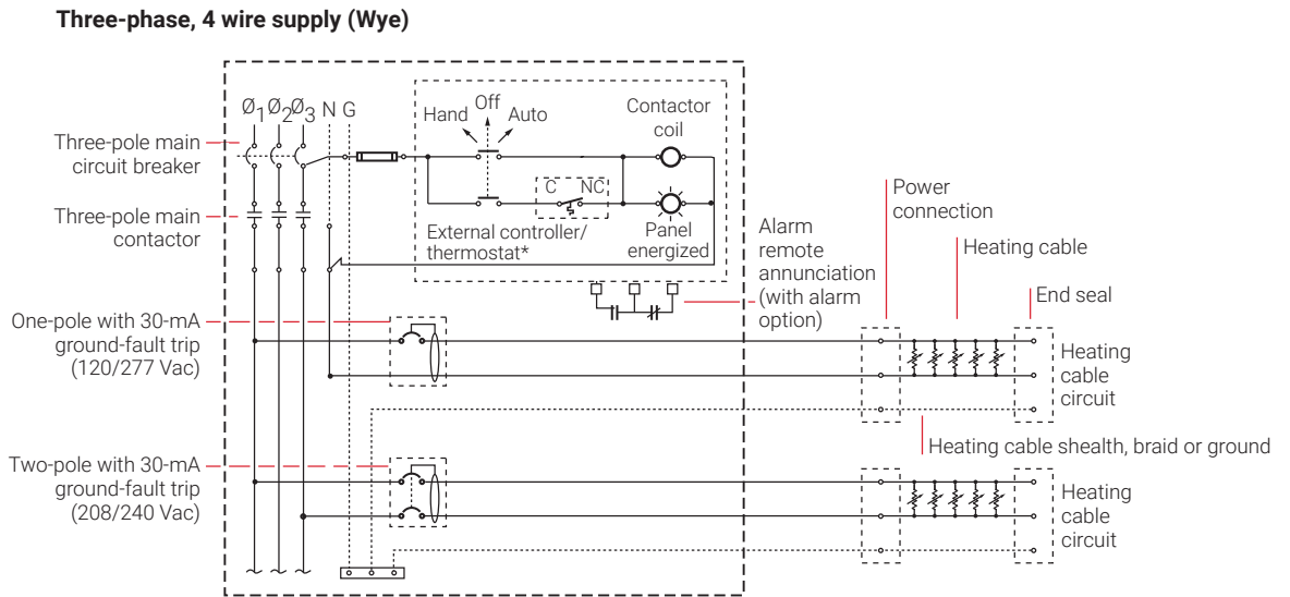
Fig. 23 Typical HTPG power schematic
