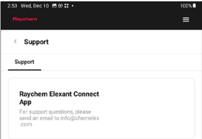
Figure 9: Support Screen
